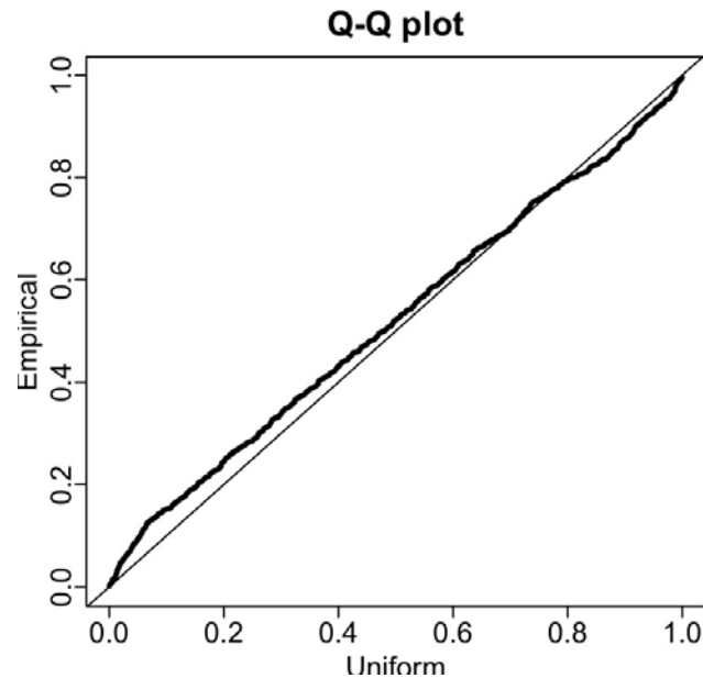
Figure 29: Quantile-quantile plot of residuals for "positive catch rate" component.
