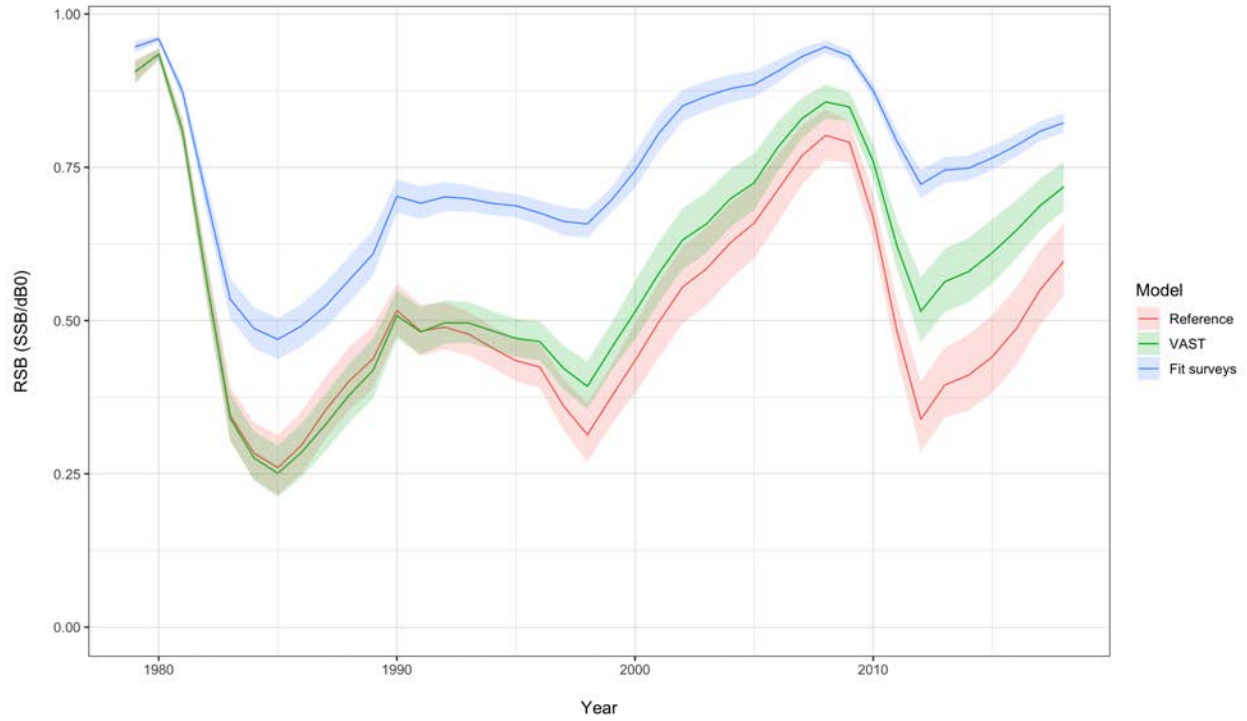
Figure 26: Comparisons of mature male biomass relative to the dynamic B_0 value, (15 February, 1978-2018) for each of the model scenarios.
