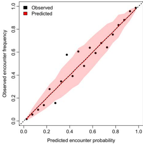
Figure 27: Observed encounter rates and predicted probabilities for SMBKC.
