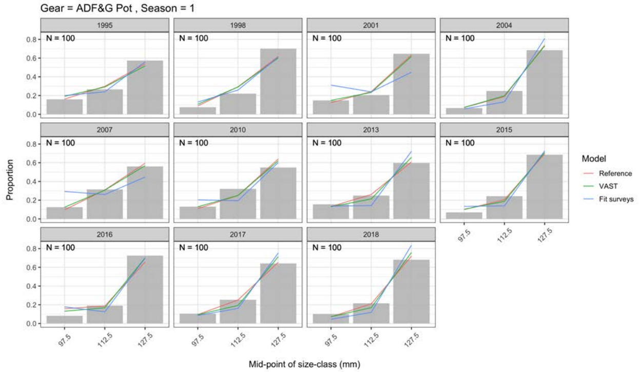
Figure 22: Observed and model estimated size-frequencies of discarded SMBKC by year in the ADF&G pot survey for the model scenarios.
