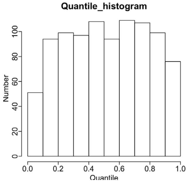
Figure 28: Plot indicating distribution of quantiles for "positive catch rate" component.
