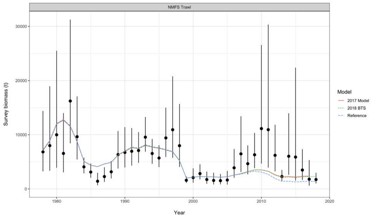
Figure 6: Fits to NMFS area-swept trawl estimates of total ( \geq 90\text{mm} ) male survey biomass with the addition of new data (the Reference Model is with all new data while 2018 BTS is just with the 2018 NMFS trawl survey data added). Error bars are plus and minus 2 standard deviations.
