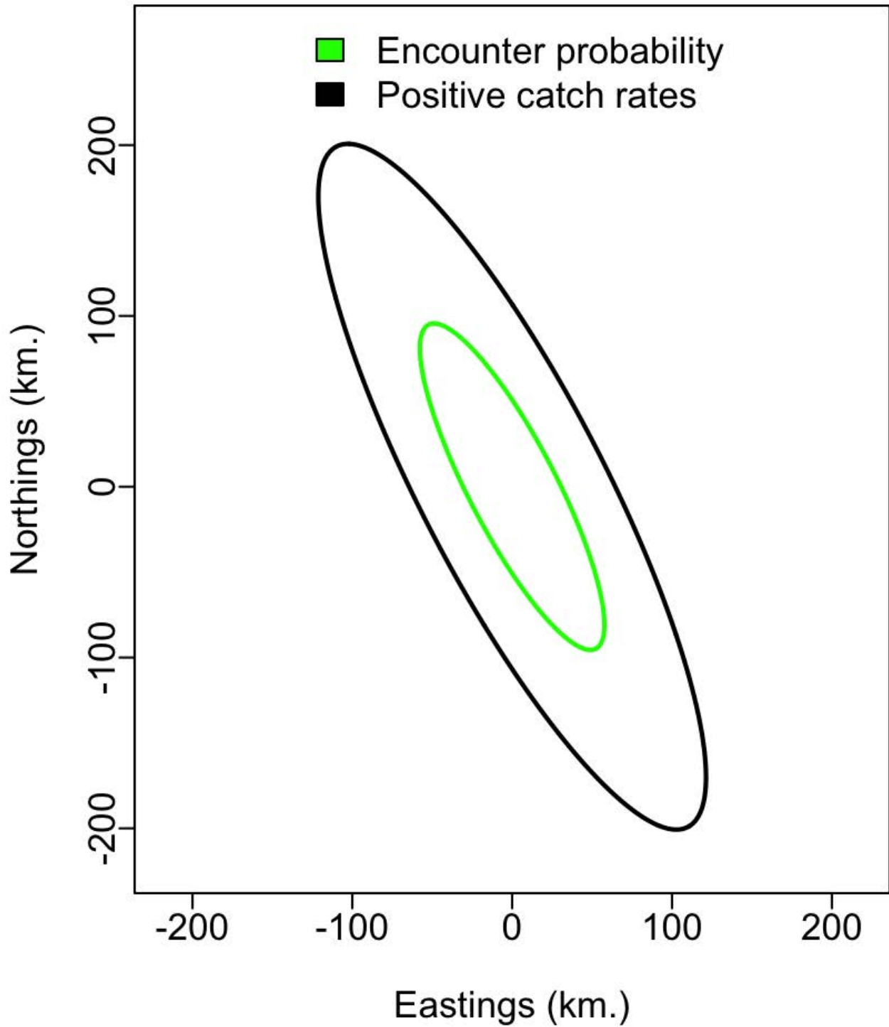
Figure 32: Directional decorrelation for SMBKC stations, 1978-2018.
