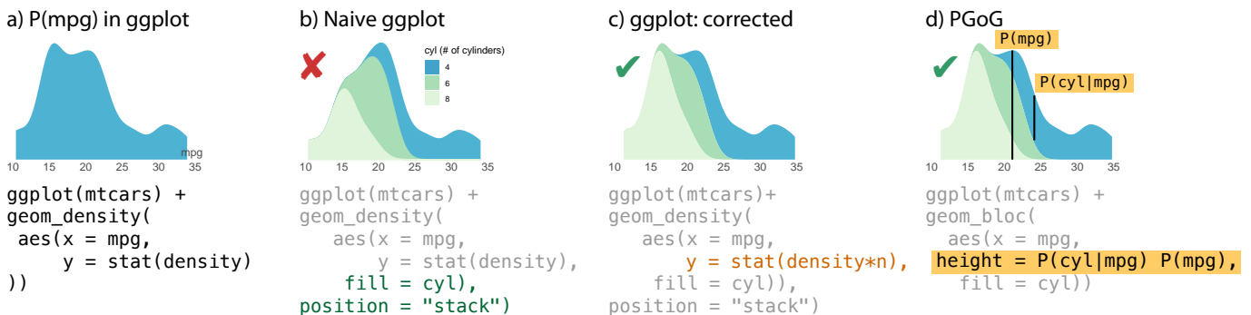
Figure 2. A motivating example for the Probabilistic Grammar of Graphics. a) For reference, a density plot for variable mpg alone: P(mpg) . b) In base ggplot2 : naively introducing the variable cyl creates partition of the density plot disproportional to the true cyl counts. c) In base ggplot2 : normalizing the colored regions by hacking internal variables ( density * n ) creates a correct stacked density plot. d) PGoG generates the correct density plot using syntax closer to users’ statistical language, in terms of probability expressions.
