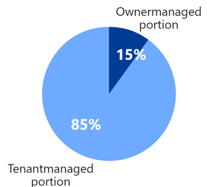
Breakdown of CO 2 emissions in 2020
