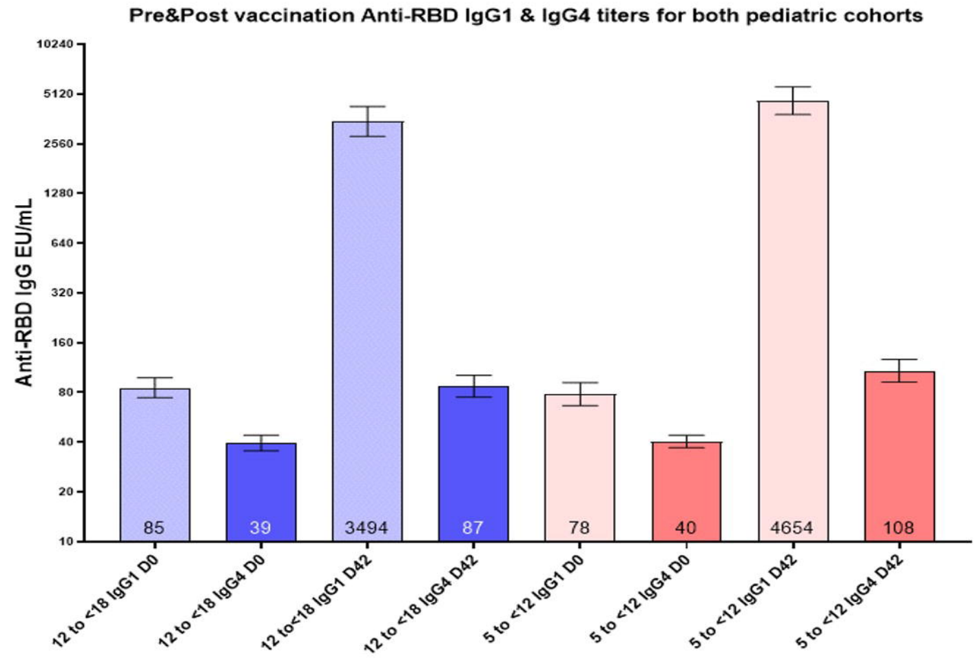
Figure 3: Summary of anti-RBD IgG sub class titers in both pediatric age sub groups: A) Anti-RBD IgG1 and IgG4 geometric mean concentrations were measured at day0 and day 42 post vaccination. In both age sub groups, IgG1 subclass titers predominantly increased after vaccination with CORBEVAX™ whereas IgG4 levels were comparable at day 0 and day 42 time points, indicating that CORBEVAX™ vaccine induces Th1 skewed immune responses. GMCT's with 95% Confidence Interval (two-sided bars) are included in the figure.
