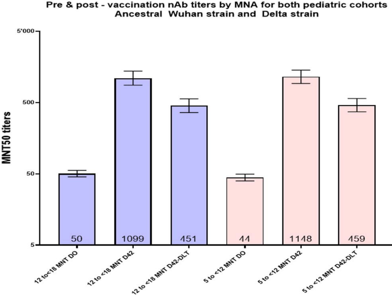
Figure 4: nAb titers measured against ancestral and Delta strains of SARS-COV-2: Neutralizing Antibody titers were tested in the subject sera samples collected prior to vaccination (Day-0) and fourteen days after two doses of vaccination (Day-42). The testing was conducted against Wild-Type SARS-COV-2 strain and Delta strain in a Micro Neutralization Assay (MNA). The observed nAb GMT's in both age groups that received CORBEVAX™ vaccine are much higher than the thresholds induced by other COVID-19 vaccines, which is indicative of >90% vaccine effectiveness of CORBEVAX™ vaccine. GMCT's with 95% Confidence Interval (two-sided bars) are included in the figure.
