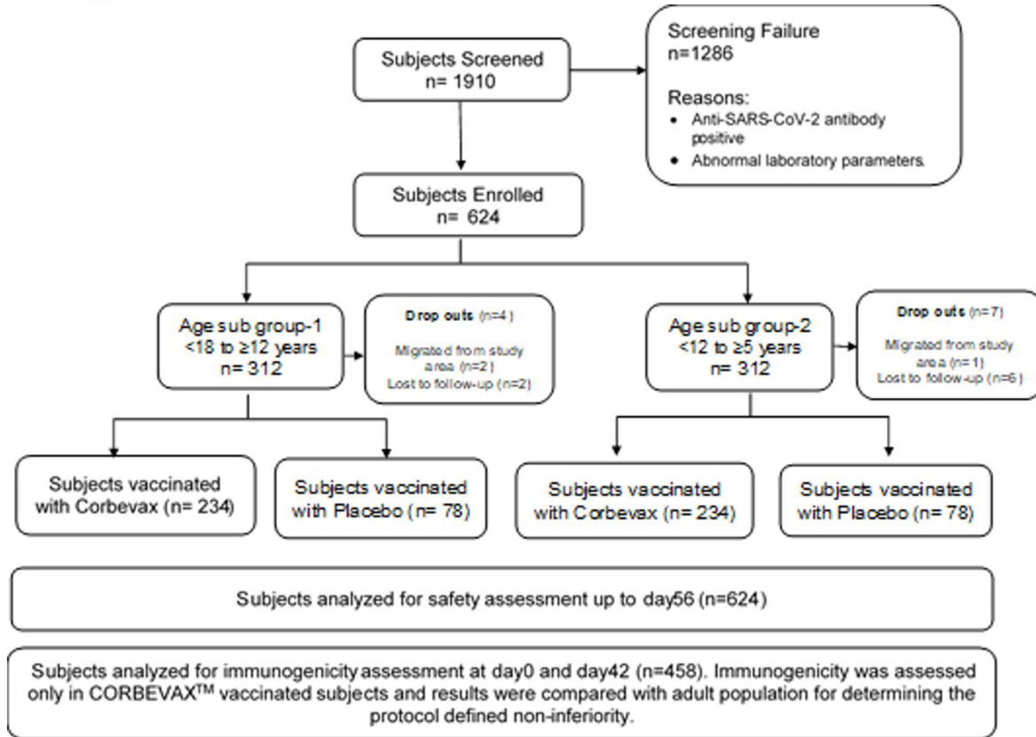
Figure 1: Subject disposition: A total of 1910 subjects were screened and 624 eligible subjects were enrolled into the study. Out of 624 subjects, 312 subjects were enrolled in <18 to ≥12 years age sub group and randomized to either CORBEVAX™ vaccination group or placebo group in a 3:1 ratio. Similar approach was followed for <12 to ≥5 years age sub group cohort (n=312). All subjects were of Indian origin and male, female ratio was balanced in both age sub groups. All the 624 subjects received two doses (0.5 ml) of either Biological E's CORBEVAX™ vaccine (468 subjects) or placebo (156 subjects) intramuscularly in the deltoid muscle of the non-dominant upper arm and completed their follow up period of Day-56. A total of 11 subjects dropped out from the study, either due to migration from study area or due to lost to follow up. All 624 subjects were assessed for safety analyses and 458 subjects out of 468 (97.8%) subjects were included in the immunogenicity assessment.
