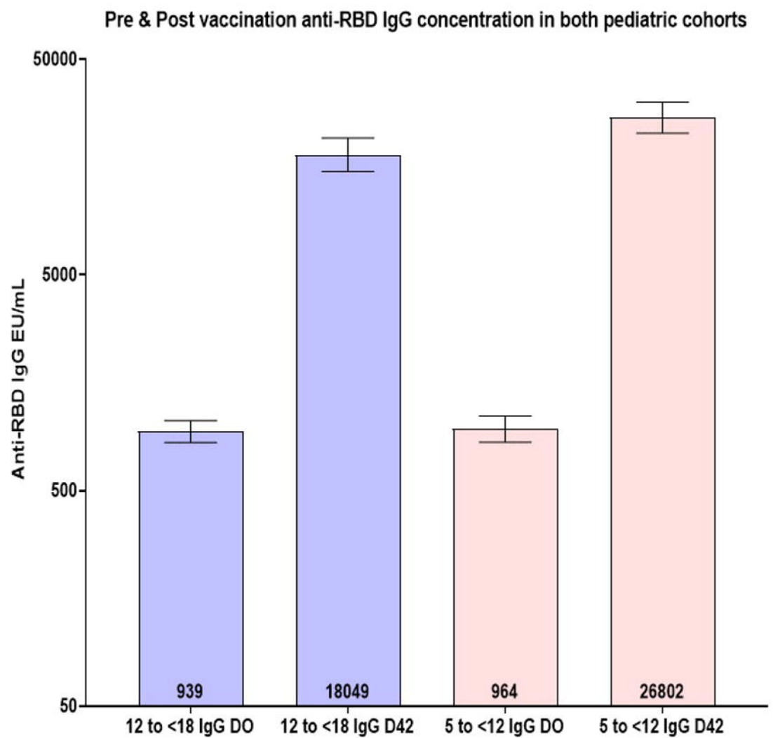
Figure 2: Summary of anti-RBD IgG concentrations in both pediatric age sub groups: A) Anti-RBD IgG concentrations were induced significantly high in CORBEVAX™ vaccinated subjects measured at day 42 in comparison to day 0. GMCT's with 95% Confidence Interval (two-sided bars) are included in the figure.
