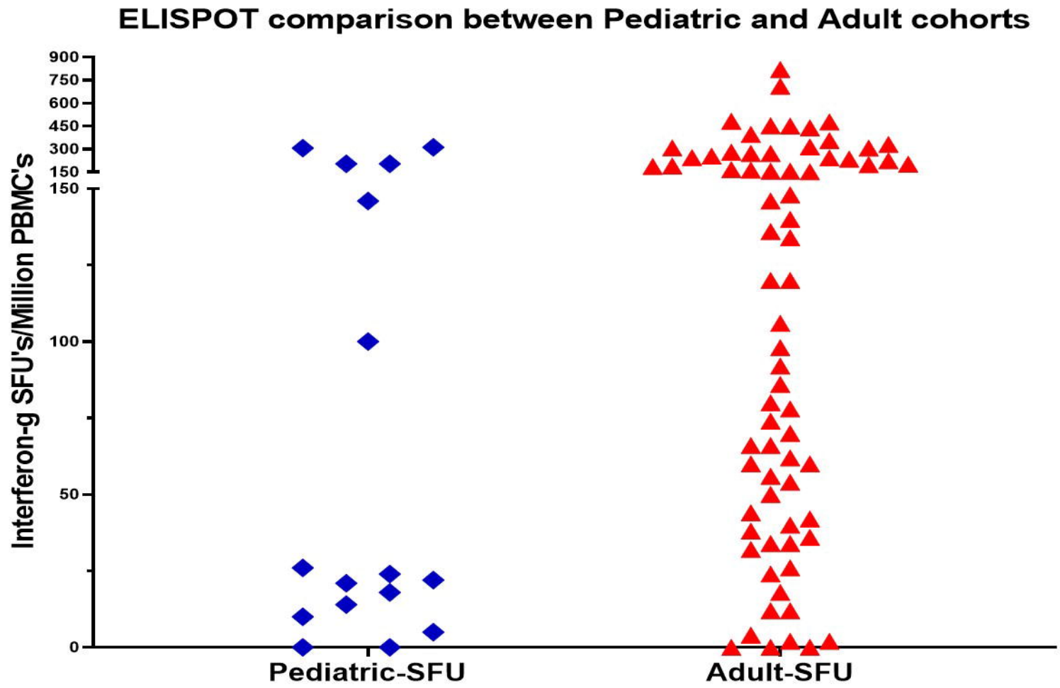
Figure 5: Comparison of cellular immune response in pediatric and adult population via ELISPOT: The total Interferon-gamma secreting PBMC's upon stimulation with SARS-COV-2 RBD peptides were measured for sixteen subjects in the pediatric population. The magnitude of cellular immune response in the pediatric cohort was similar to the adult population in terms of Interferon-gamma ELISPOT SFU's
