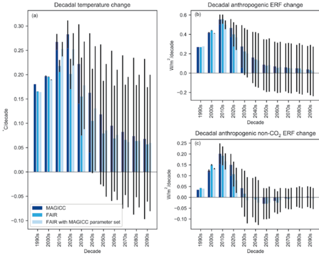
Figure 2.SM.1 | Warming rates per decade for MAGICC (dark blue), FAIR (sky blue) and FAIR matching the MAGICC parameter set (light blue) for the scenario dataset used in this report. These bars represent the mean of regression slopes taken over each decade (years 0 to 9) for scenario median temperature changes, over all scenarios. The black bars show the standard deviation over the set of scenarios.
