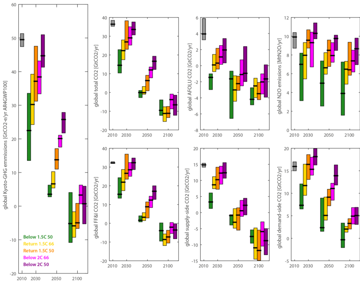
1 2 Figure 2.8: Annual global emissions characteristics of five scenario classes used in this chapter for 2010, 2030, 2050, 3 2100 for Kyoto-GHG emissions (left-most panel), total CO 2 emissions, CO 2 emissions from the AFOLU 4 sector, and global N 2 O emissions (top row), as well as CO 2 emissions from fossil-fuel use and industrial 5 processes. The latter is also split into emissions from the energy supply sector (electricity sector and 6 refineries), and direct emissions from fossil fuel use in energy demand sectors (industry, buildings, 7 transport) (bottom row panels). Boxes with different colours refer to different scenario classes (see left 8 panel). Ranges in the bottom panels show the interquartile range, horizontal black lines the median.
