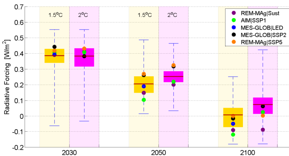
Figure 2.10: Radiative forcing from fluorinated (F) gases and ozone depleting substances (ODS), short-lived climate forcers including methane, tropospheric ozone, and aerosols (net total of sulphate, nitrate, organic
