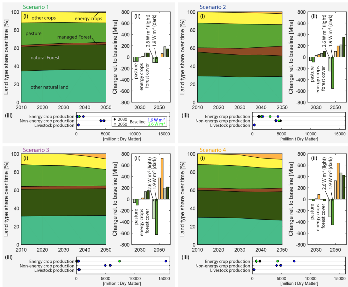
Figure 2.28: Four land pathway types for land transitions consistent with 1.5°C. 1.9 and 2.6 W m^{-2} are taken as a proxy for 1.5°C and 2°C scenarios, respectively. 2.6 W m^{-2} scenarios are mostly consistent with the ‘below 2C 66’ and ‘below 2C 50’ scenarios classes. 1.9 W m^{-2} scenarios are consistent with ‘return 1.5C 66’ scenario class. Each square illustrates the characteristics of one particular illustrative scenario and shows: (i) a temporal evolution until 2050 of the share of various land types in 1.9 W m^{-2} scenarios; (ii) change of land surface for three land types (pasture, energy crops, and forest cover) relative to a no-climate mitigation baseline for 2.6 W m^{-2} (lighter bars) and 1.9 W m^{-2} (darker bars) scenarios, respectively, in 2030 and 2050; (iii) production indicators in 2030 (diamonds) and 2050 (circles) for the baseline, 2.6 W m^{-2} and, 1.9 W m^{-2} scenarios. Data from (Riahi et al., 2017; Rogelj et al., 2017b). Colours of scenario names link back to the colour of single scenario symbols in Figure 2.27. Due to differences in base year data sources, and large uncertainties in historical data, land-use patterns differ between the models already in 2010 (Alexander et al., 2017; Popp et al., 2017; Prestele et al., 2016).
