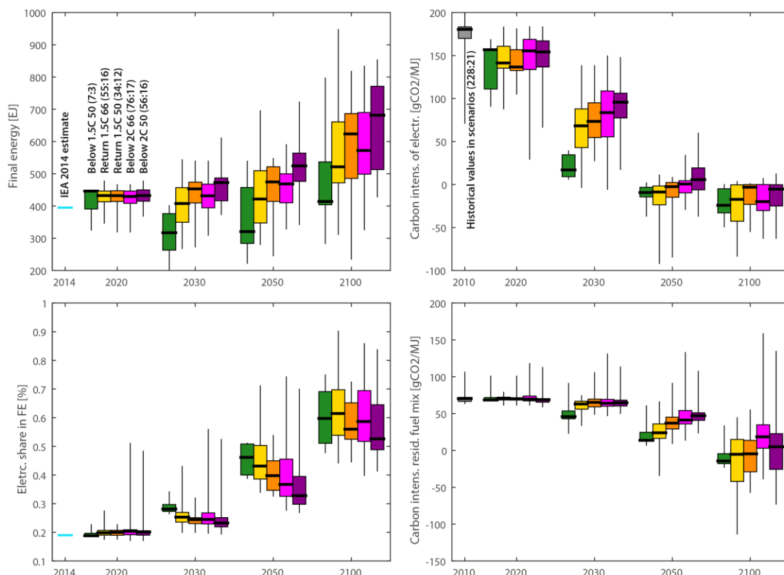
11 Figure 2.11: Decomposition of transformation pathways in energy demand (top left: EJ of final energy), carbon 12 intensity of electricity (top right: Electricity CO 2 over Electricity in Final Energy), the electricity 13 share in final energy (bottom left), and the carbon intensity of the residual (non-electricity) fuel 14 mix (bottom right). Boxplots show median, interquartile range and full range. The legend for the 15 scenario classes is provided in the top left panel. Values behind the class labels report the number 16 of available scenarios and the number of contributing modelling framework. Classes are defined in 17 Section 2.1. Historical values in the left panels are from IEA (IEA, 2016b). 18 19 20
