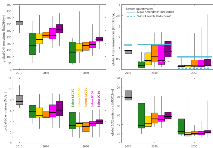
24 25 Figure 2.9: Global characteristics of a selection of global short-lived non-CO 2 emissions until mid-century for five 26 scenario classes used in this chapter in terms of annual emissions levels in 2010, 2030, and 2050. Data is 27 shown for methane (CH 4 ), fluorinated gases (F-gas), black carbon (BC), and sulphur dioxide (SO 2 ) 28 emissions. Boxes with different colours refer to different scenario classes (defined in the bottom left 29 panel). Ranges in the bottom panels show the interquartile range, horizontal black lines the median, while 30 vertical thin lines the minimum maximum range. F-gases are expressed in units of CO 2 -equivalence 31 computed with 100-year Global Warming Potentials reported in IPCC AR4. Horizontal blue lines in the 32 top right HFC F-gas panel indicate estimates of F-gas emissions under implementation of the Kigali 33 Amendment (solid) or under implementation of the “most feasible reductions” identified by (Höglund- 34 Isaksson et al., 2017). 35
