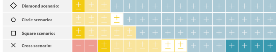
Figure 2.31: Interactions of individual mitigation measures and alternative mitigations portfolios for 1.5°C with Sustainable Development Goals (SDGs). The assessment of interactions between mitigation measures and individual SDGs is based on the assessment of Section 5.4. 7
