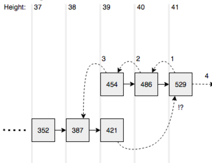
Figure 4: Fork with cumulative difficulties
